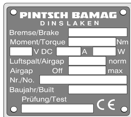
Rating plate
